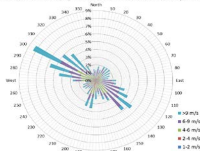
1/2 hr Maximum Wind Speed and Direction Saskatoon April 2019
