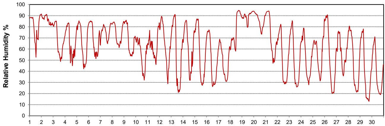
Relative Humidity for April 2023
