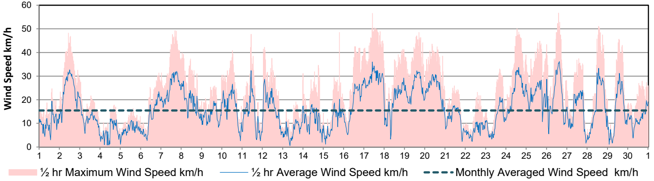
Wind Speed for April 2023
