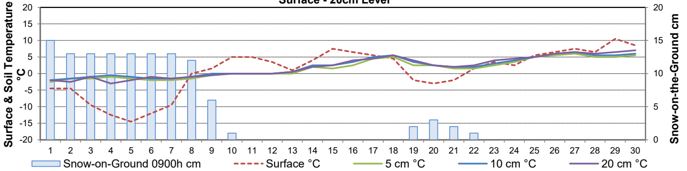
Soil Temperatures for April 2023 Surface - 20cm Level
