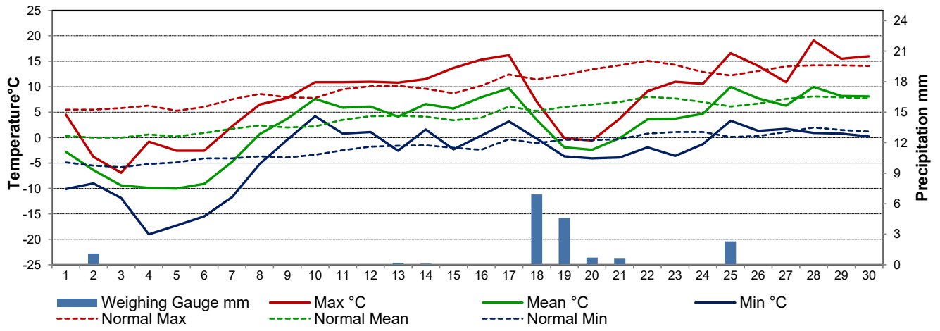
Temperature and Precipitation for April 2023
