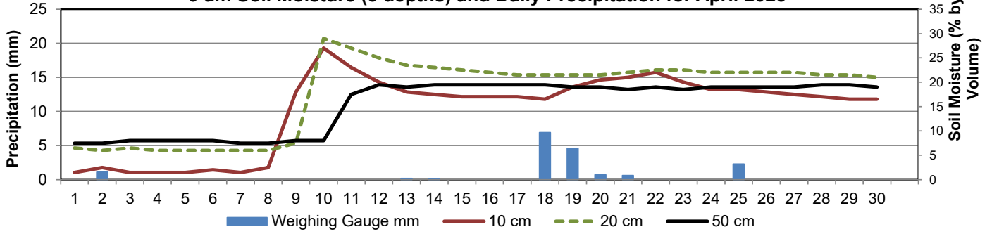
9 am Soil Moisture (3 depths) and Daily Precipitation for April 2023
