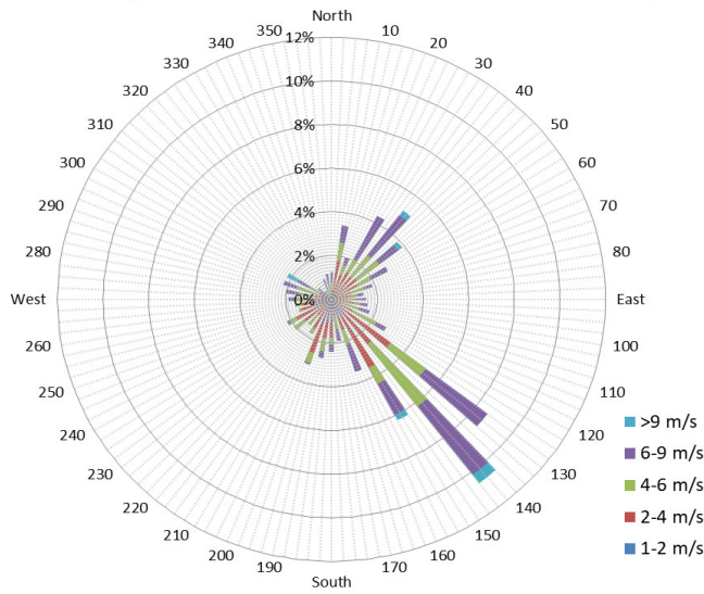
10 minute Average Wind Speed and Direction Saskatoon Apr 2023
