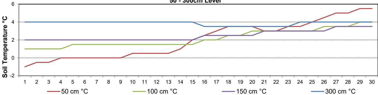
Soil Temperatures for April 2023 50 - 300cm Level
