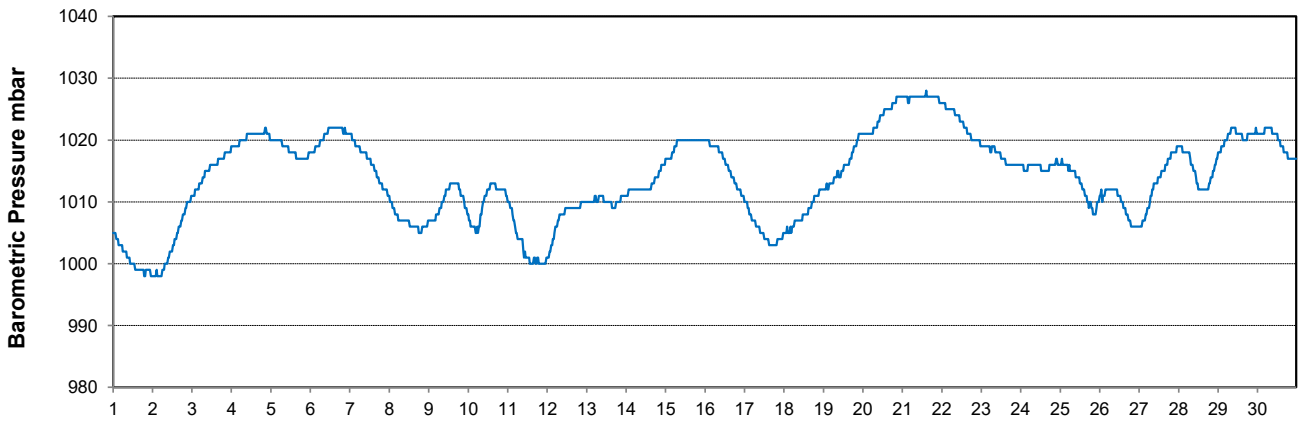
Barometric Pressure Corrected to Sea Level for April 2023
