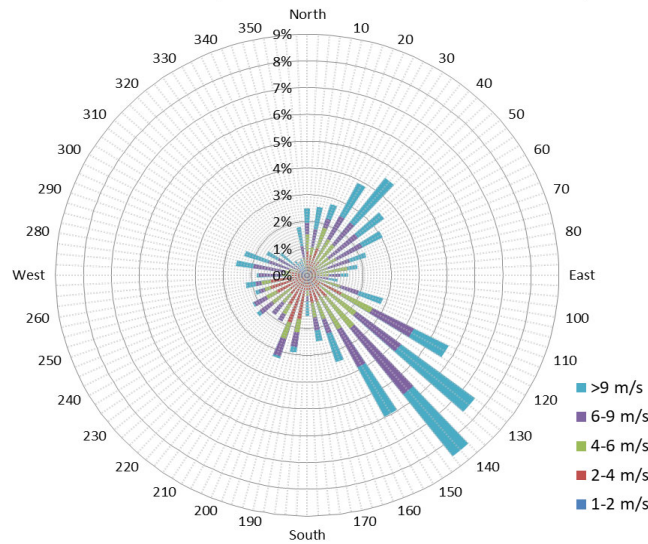
1/2 hr Maximum Wind Speed and Direction Saskatoon April 2023
