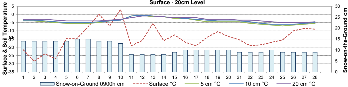
Soil Temperatures for February 2022 Surface - 20cm Level
