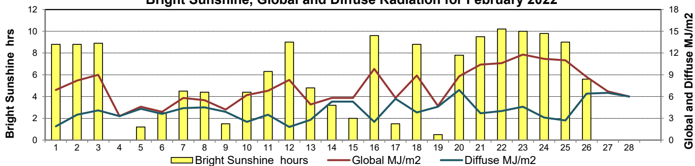
Bright Sunshine, Global and Diffuse Radiation for February 2022
